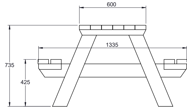
TYPICAL ELEVATION
